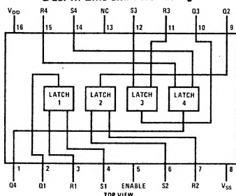
CD4043BM/CD4043BC Dual-In-Line and Flat Packages
