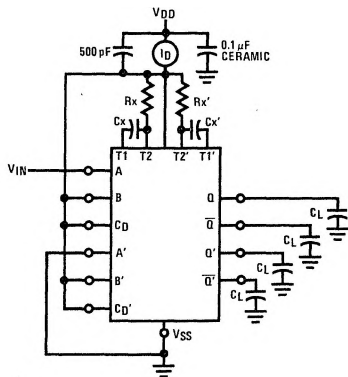
Figure 1. Power Dissipation Test Circuit and Waveforms
