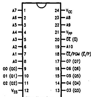
24-Pin EPROM Socket
