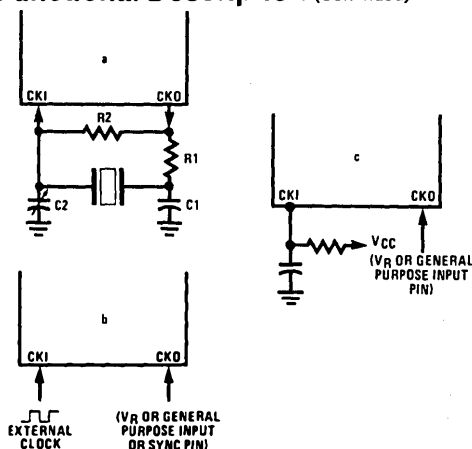
Crystal Oscillator
