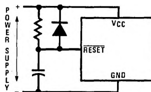
FIGURE 4. Recommended Reset Circuit
