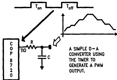
FIGURE 12. Timer Application
