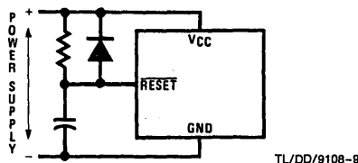
FIGURE 5. Recommended Reset Circuit
