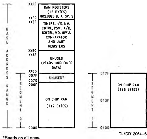
FIGURE 4. RAM Organization
