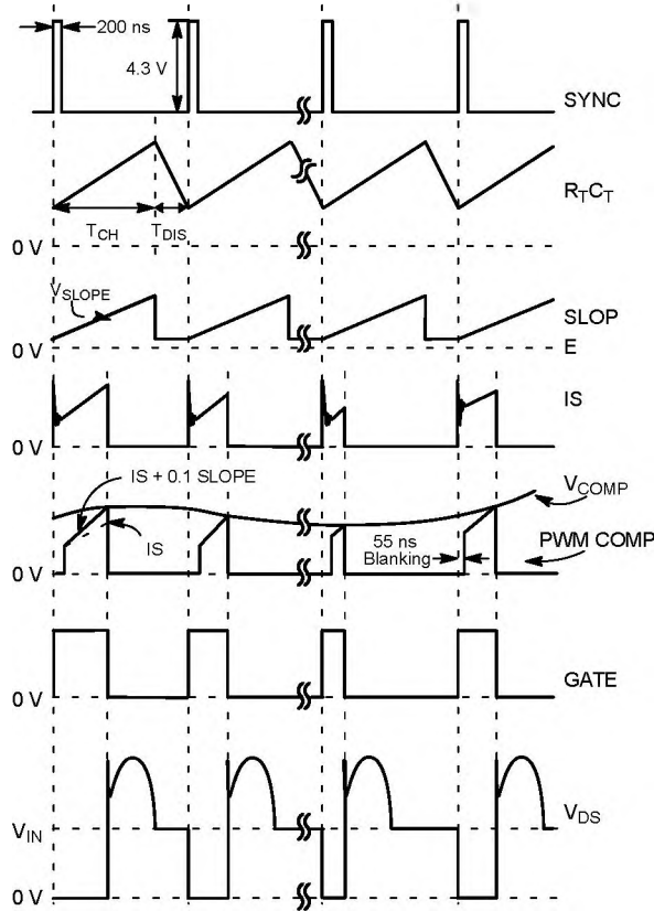
Figure 3. Typical Waveforms
