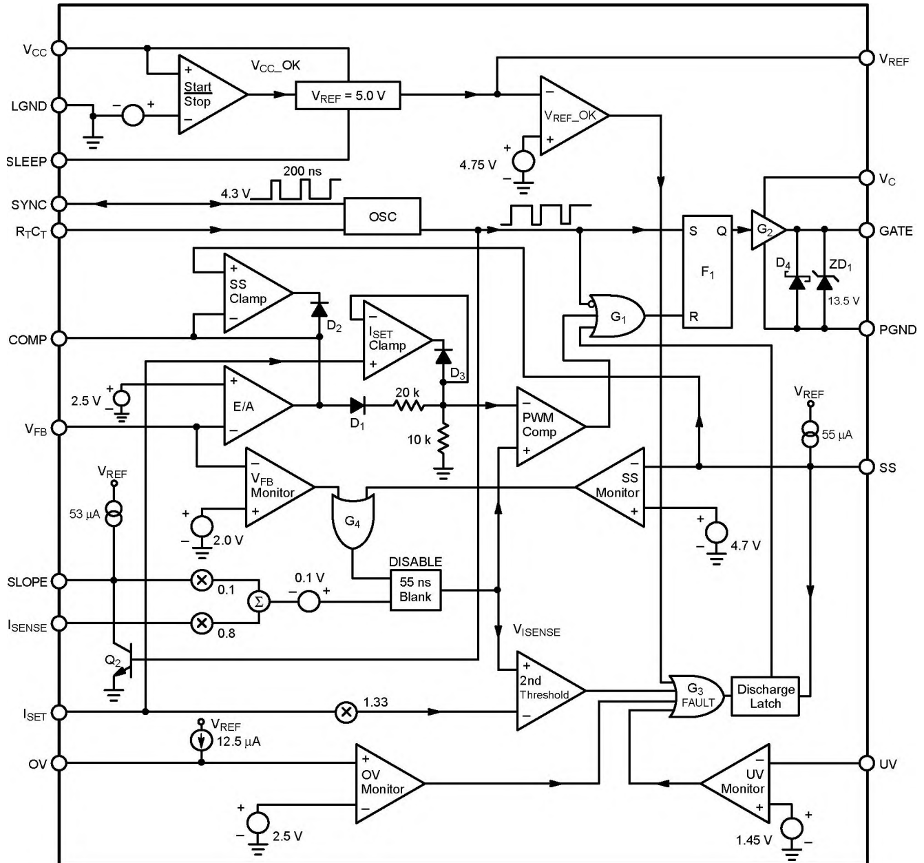
Figure 2. Block Diagram
