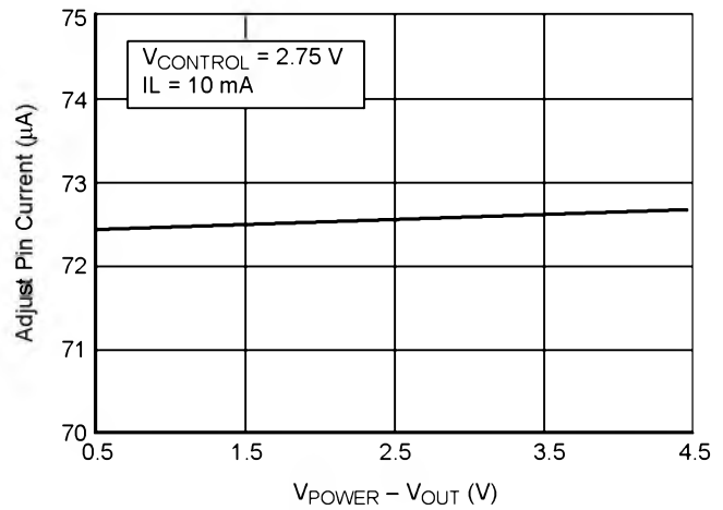
Figure 14. Adjust Pin Current vs V_{\text{POWER}} - V_{\text{OUT}}
