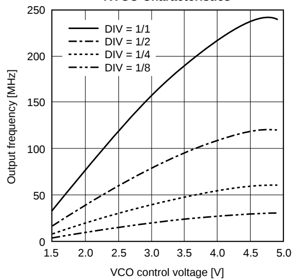
KVCO Characteristics
