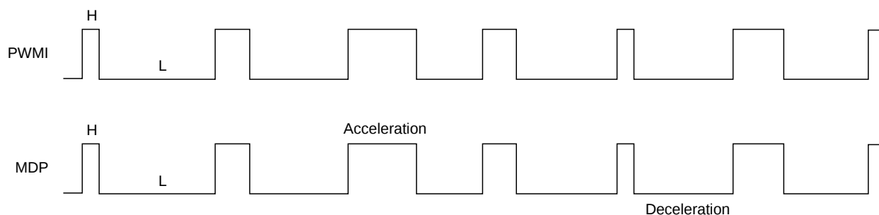
Timing Chart 1-20
