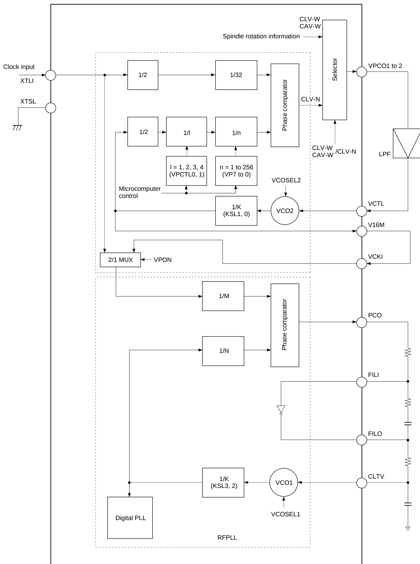
Block Diagram 4-1
