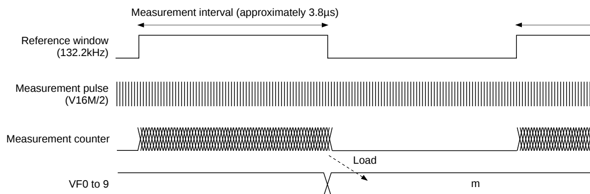
Timing Chart 2-5
