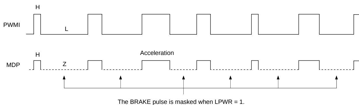
Timing Chart 1-20
