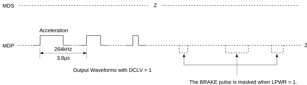
Timing Chart 1-17
