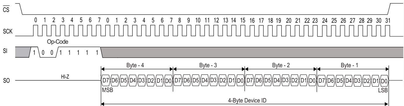
Figure 27. RDID Instruction
