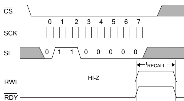
Figure 38. Software RECALL Cycle [26]
