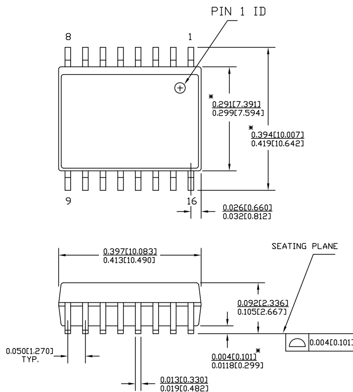
Figure 42. 16-pin SOIC (0.413 × 0.299 × 0.0932 Inches) Package Outline, 51-85022
