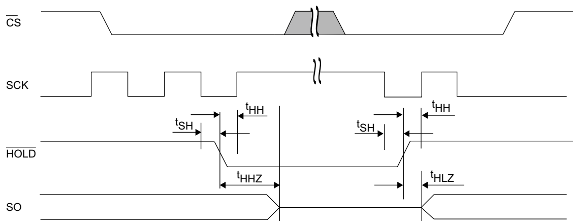
Figure 35. \overline{\text{HOLD}} Timing
