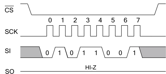
Figure 21. AutoStore Enable Operation
