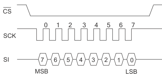
Figure 5. SPI Mode 3
