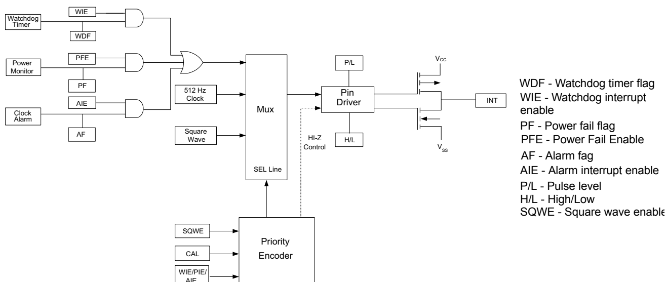
Figure 38. Interrupt Block Diagram
