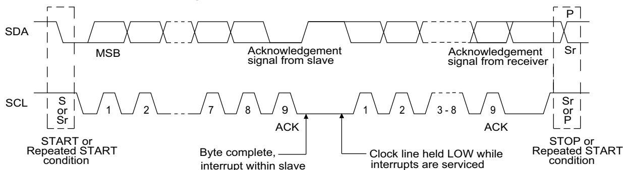
Figure 4. Data Transfer on the I 2 C Bus
