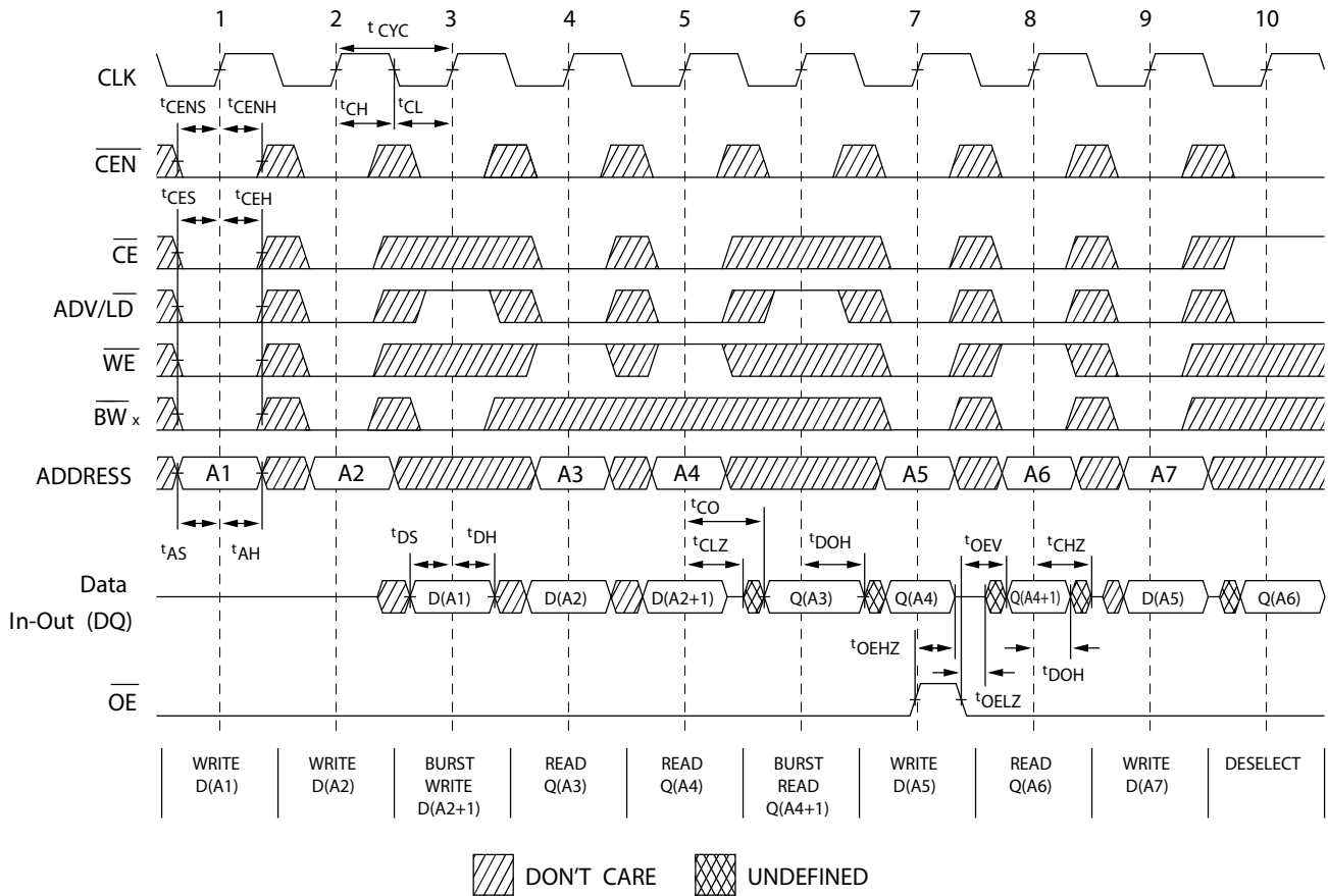
Figure 4. Read/Write/Timing [27, 28, 29]
