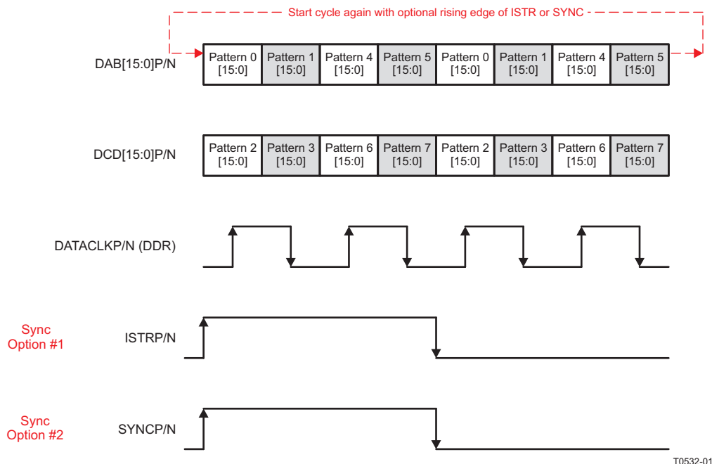
Figure 77. IO Pattern Checker Data Transmission Format
