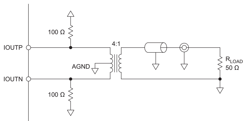
Figure 87. Driving a Doubly Terminated 50 \Omega Cable Using a 4:1 Impedance Ratio Transformer
