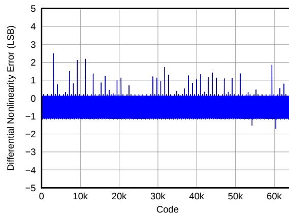
Figure 2. Differential Nonlinearity
