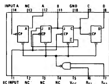
DM5492/DM7492
