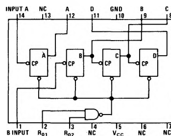
DM5493/DM7493
