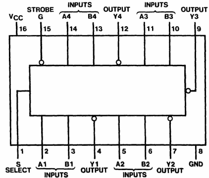
Dual-In-Line Package
