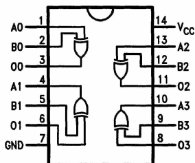
Dual-In-Line Package
