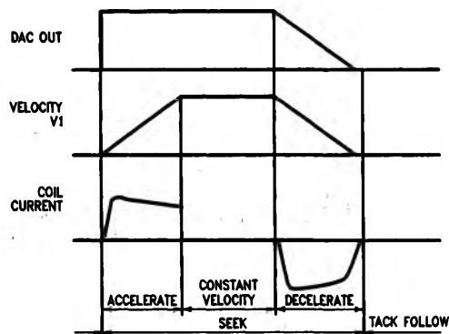
FIGURE 4. Typical Seek
