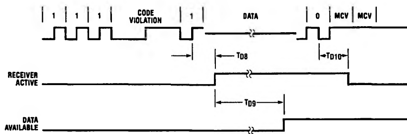
FIGURE 10. Message Timing
