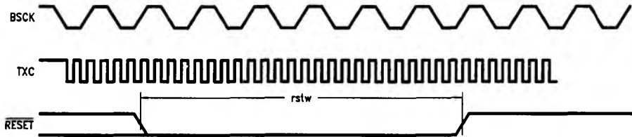
Reset Timing
