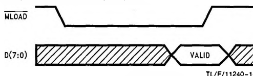
FIGURE 5-8. MLOAD Operation
