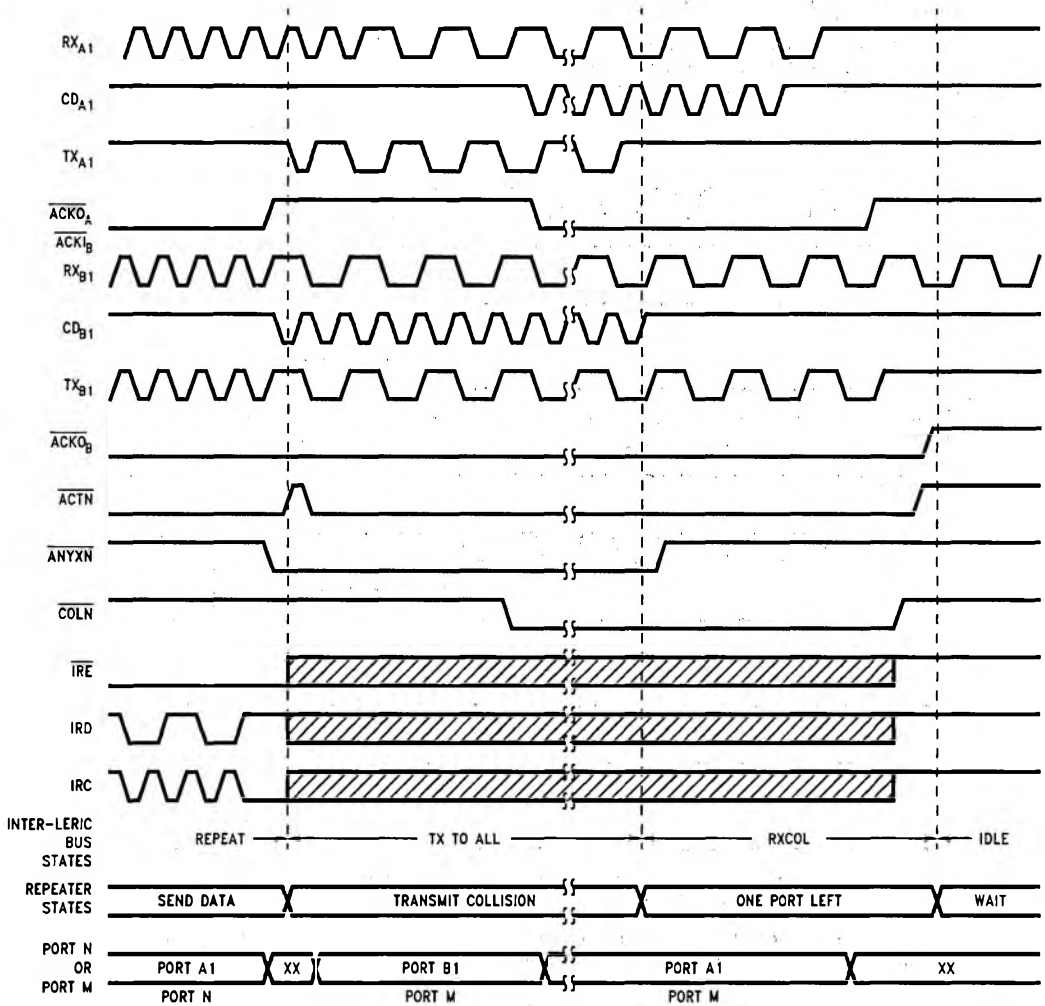
FIGURE 5-6. Transmit Collision
