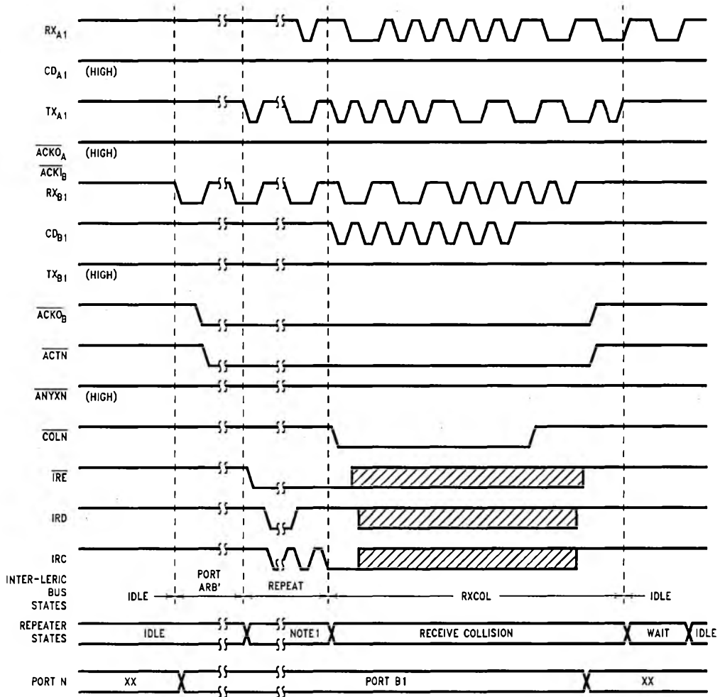
FIGURE 5-5. Receive Collision
