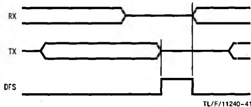
FIGURE 5-11. DFS Operation
