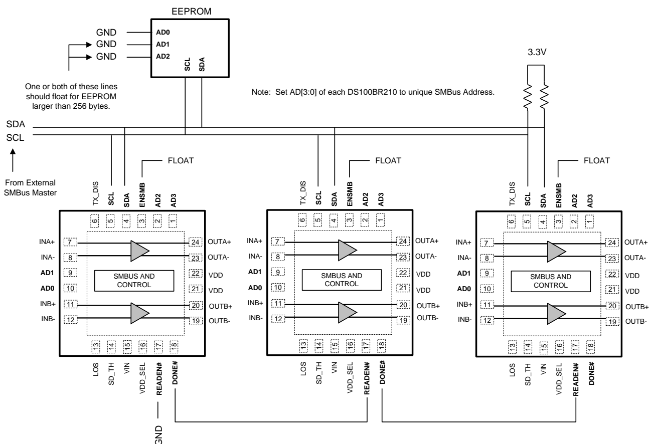
Figure 8. Typical multi-device EEPROM connection diagram
