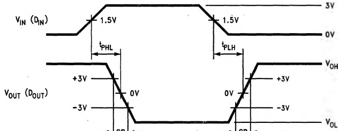
FIGURE 2. Driver Switching Waveform
