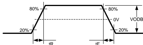
Figure 2. Driver Output Transition Time
