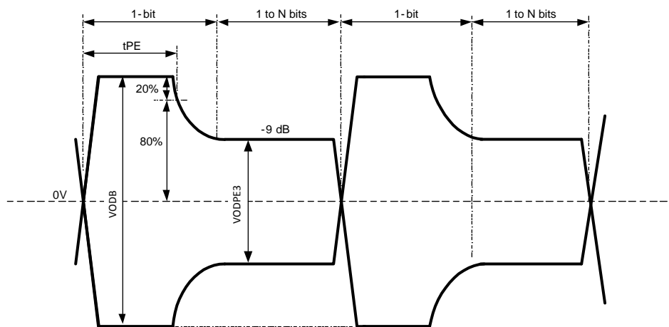
Figure 4. Test Condition for Output Pre-Emphasis Duration
