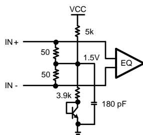
Figure 6. Receiver Input Termination and Bias Circuit
