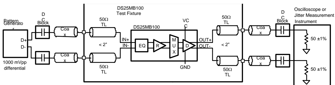
Figure 5. AC Test Circuit
