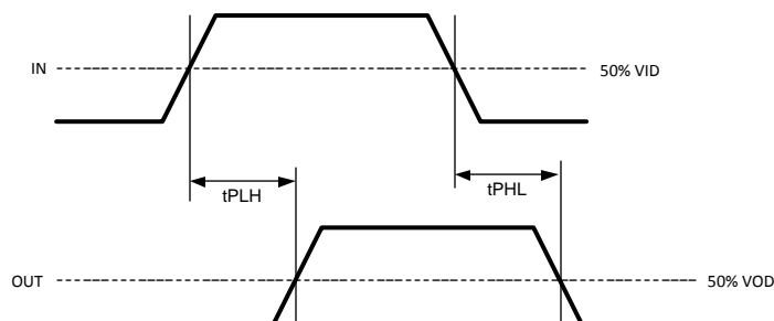
Figure 3. Propagation Delay from Input to Output
