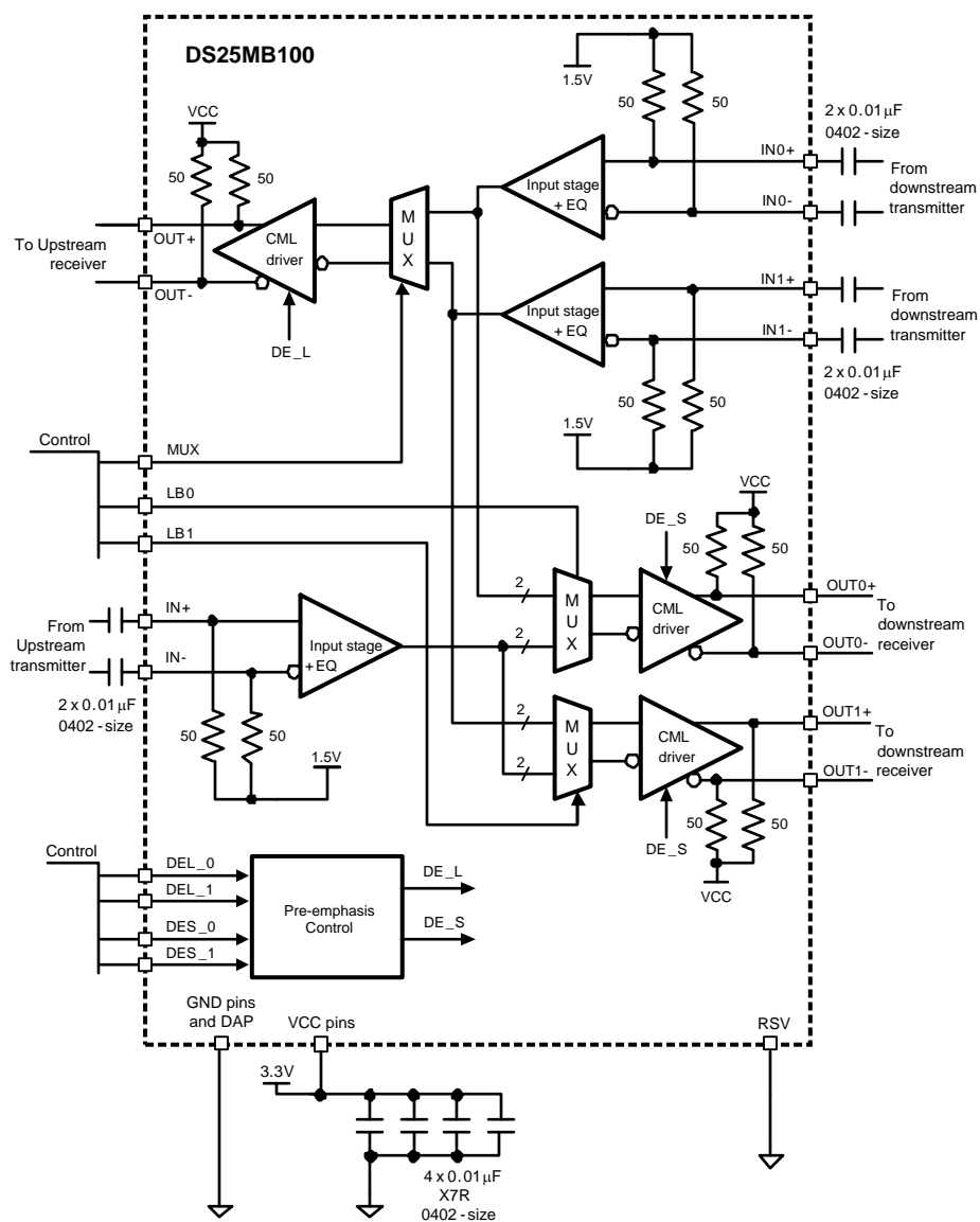
Figure 7. Application Diagram
