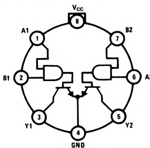
TL/F/5824-7
