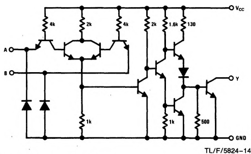
DS55454/DS75454
