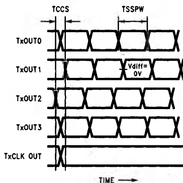
FIGURE 6. DS90CF581 (Transmitter) Channel-to-Channel Skew and Pulse Width
