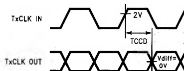
FIGURE 9. DS90CR581 (Transmitter) Clock In to Clock Out Delay
