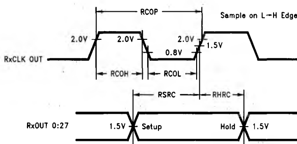
FIGURE 8. DS90CR582 (Receiver) Setup/Hold and High/Low Times
