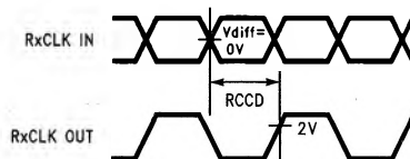
FIGURE 10. DS90CR582 (Receiver) Clock In to Clock Out Delay
