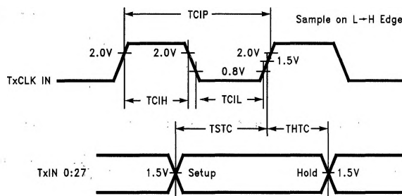
FIGURE 7. DS90CR581 (Transmitter) Setup/Hold and High/Low Times
