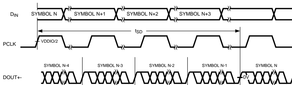
Figure 14. Serializer Delay
