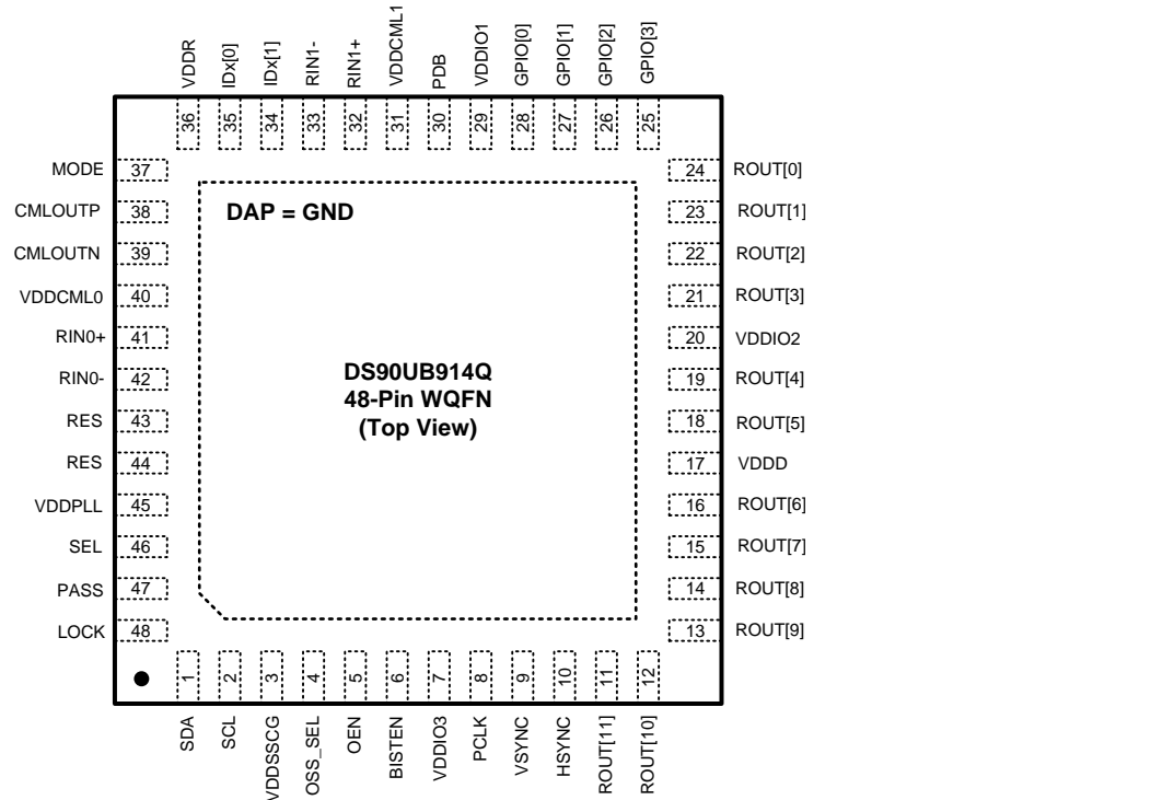
Deserializer - DS90UB914Q — Top View
