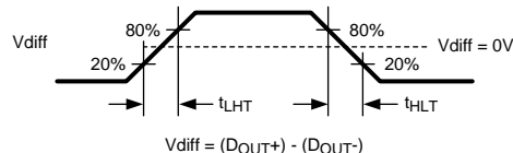
Figure 6. Serializer CML Output Load and Transition Times
