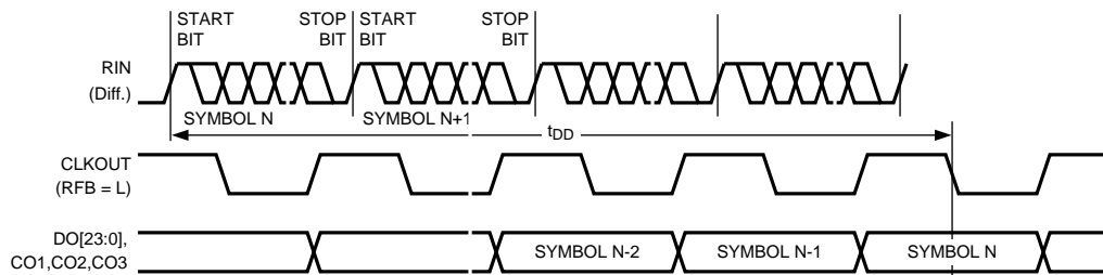
Figure 13. Deserializer Delay – Latency
