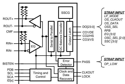
DS92LV2422 – DESERIALIZER
