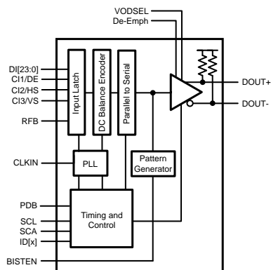
DS92LV2421 – SERIALIZER
