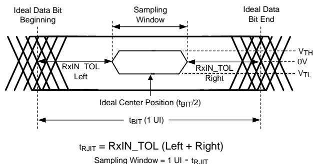
Figure 18. Receiver Input Jitter Tolerance
