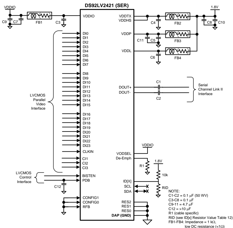
Figure 34. DS92LV2421 Typical Connection Diagram — Pin Control
