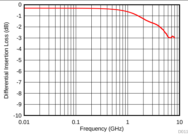
Figure 9. Differential Insertion Loss
