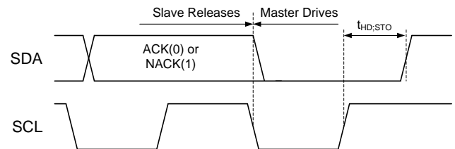
Figure 39. Stop Bit
