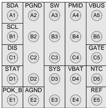
Figure 3. Top View
