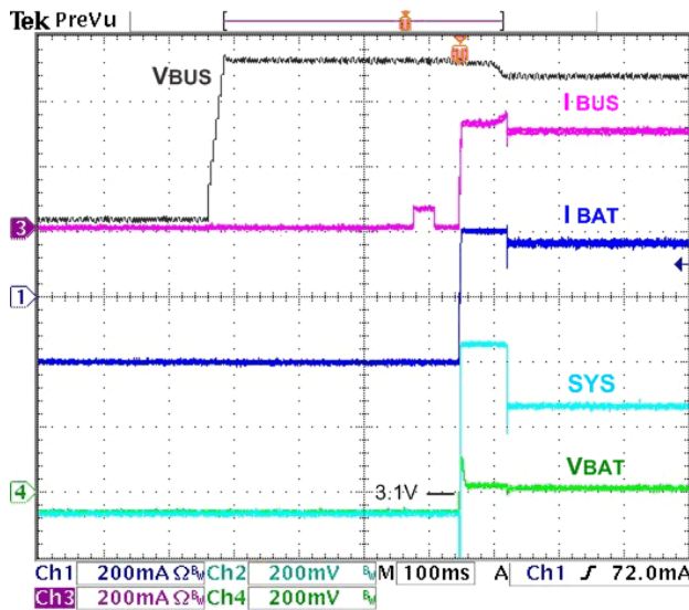
Figure 15. Charger Startup at V_{\text{BUS}} Plug-In Using 300 mA Current Limited Source, 500 mA I_{\text{BUSLIM}} , 3.1 V_{\text{BAT}} , 200 mA SYS Load, CE# = 0, IO_LEVEL = 0
