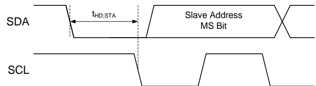
Figure 38. Start Bit
