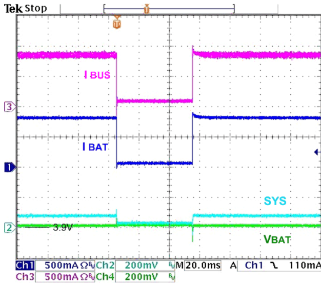
Figure 17. Battery Removal / Insertion while Charging, TE = 0 , 3.9\text{ V}_{BAT} , I_{OCHARGE} = 950\text{ mA} , I_{BUSLIM} = \text{No Limit} , 50\ \Omega\text{ SYS Load}
