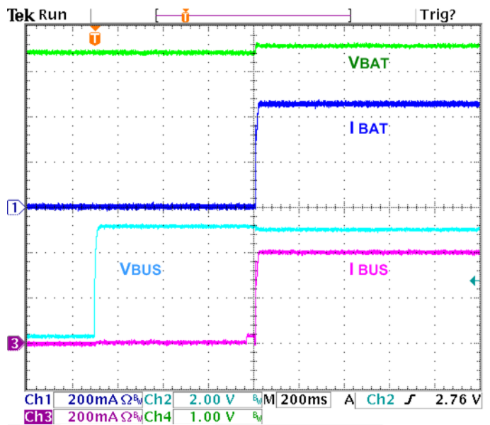
Figure 13. Auto-Charge Startup at V_{BUS} Plug-in, I_{INLIM}=500\text{ mA} , OTG=1 , V_{BAT}=3.4\text{ V}
