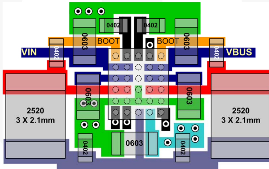
Figure 54. Recommended Layout for High-Current Charging, Using 2520 Inductors
