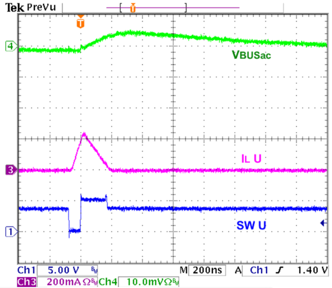
Figure 39. Boost PFM Waveform
