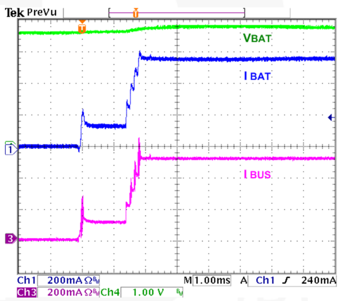
Figure 15. Charger Startup with HZ\_MODE Bit Reset, I_{INLIM}=500\text{ mA} , I_{OCHARGE}=950\text{ mA} , V_{OREG}=4.2\text{ V} , V_{BAT}=3.6\text{ V}
