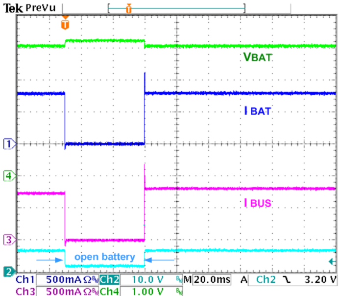
Figure 16. Battery Removal / Insertion during Charging, V_{BAT}=3.9\text{ V} , I_{OCHARGE}=950\text{ mA} , No I_{NLIM} , TE=0
