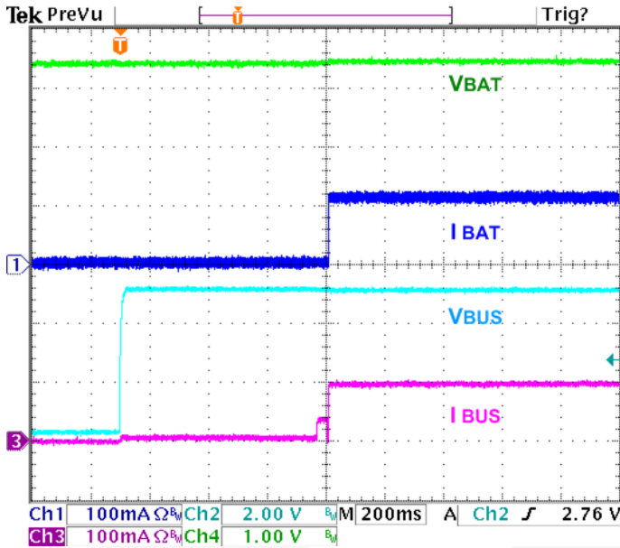
Figure 12. Auto-Charge Startup at V_{BUS} Plug-in, I_{INLIM}=100\text{ mA} , OTG=1 , V_{BAT}=3.4\text{ V}
