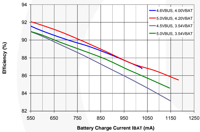
Figure 10. Charger Efficiency, No I_{INLIM} , I_{OCHARGE}=1250\text{ mA}
