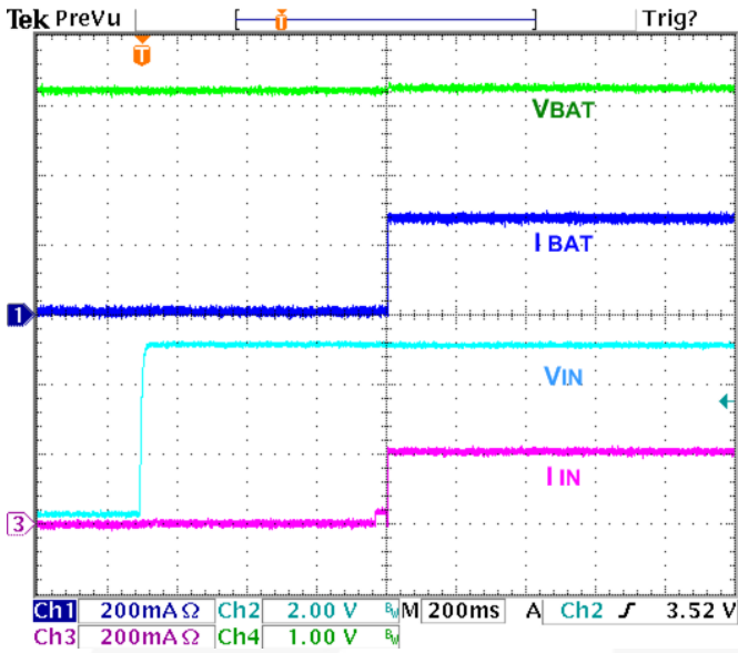
Figure 24. Auto-Charge Startup at V_{IN} Plug-in, V_{BAT}=3.2\text{ V} , I_{O\_LEVELV} = 1
