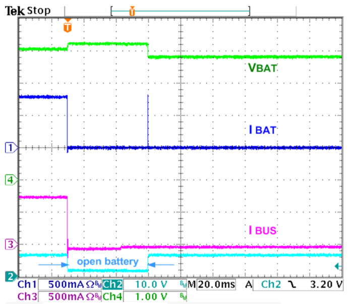
Figure 17. Battery Removal / Insertion during Charging, V_{BAT}=3.9\text{ V} , I_{OCHARGE}=950\text{ mA} , No I_{NLIM} , TE=1
