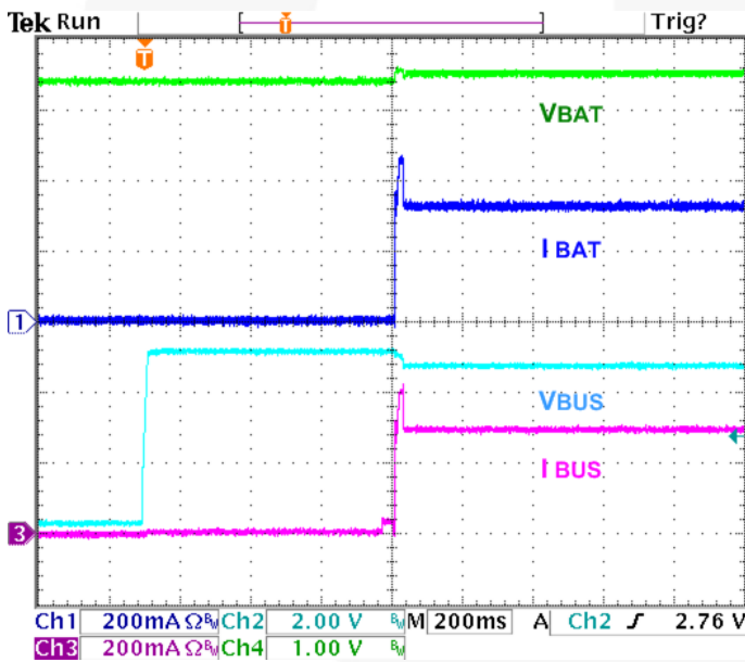
Figure 14. AutoCharge Startup with 300 mA Limited Charger / Adaptor, I_{INLIM}=500\text{ mA} , OTG=1 , V_{BAT}=3.4\text{ V}
