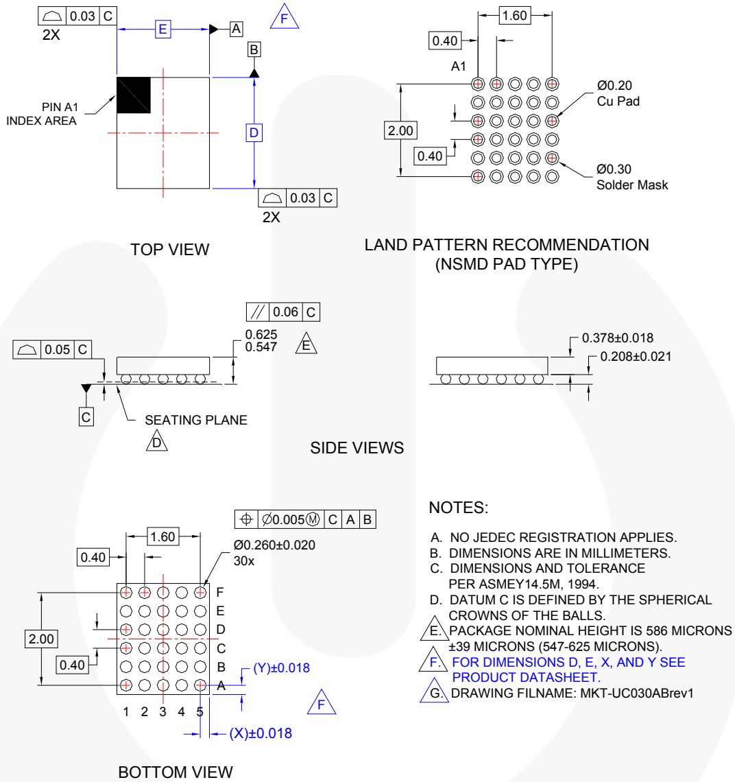
Figure 61. 30-Ball, WLCSP, 5x6 Array, 0. mm Pitch, 586 µm Package Height
