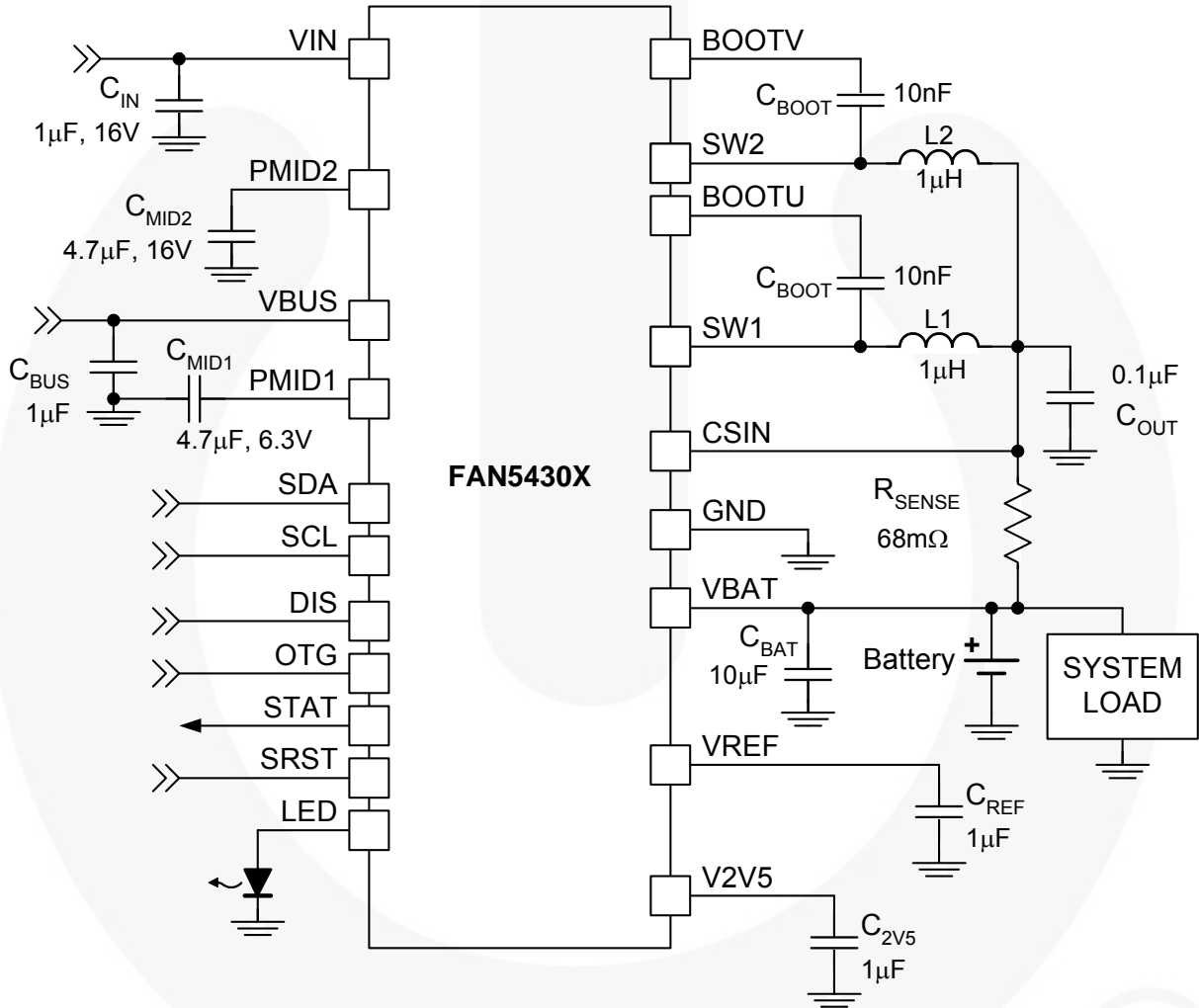
Figure 1. Typical application
