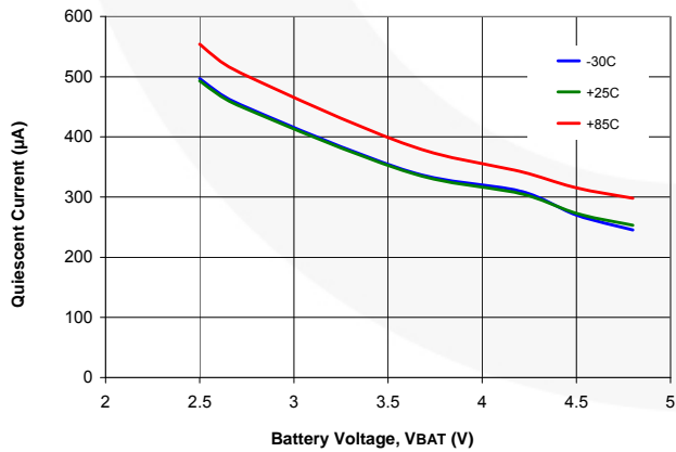
Figure 36. Quiescent Current
