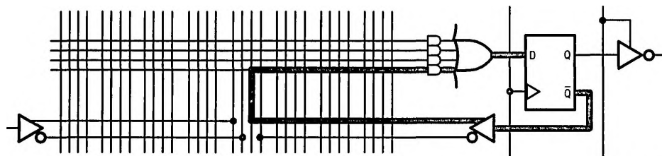
Typical Registered Logic Function With Feedback
