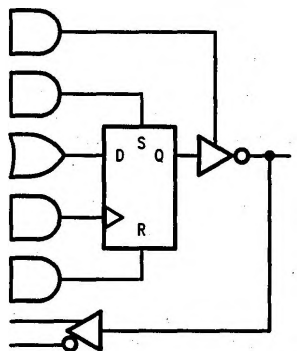
Registered/Active Low
