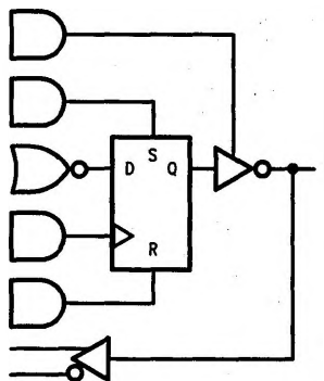
Registered/Active High
