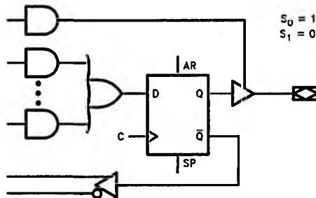
FIGURE 3-2. Registered/Active High
