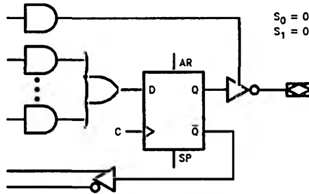
FIGURE 3-1. Registered/Active Low
