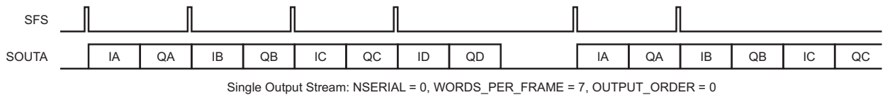
Figure 1-15. Serial Output Formats
