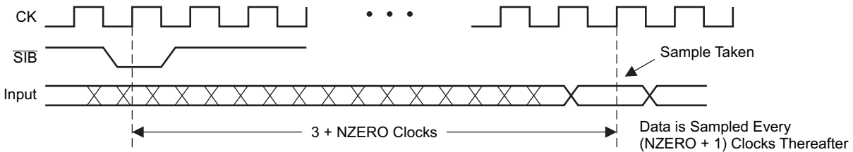
Figure 1-5. Zero-Pad Synchronization
