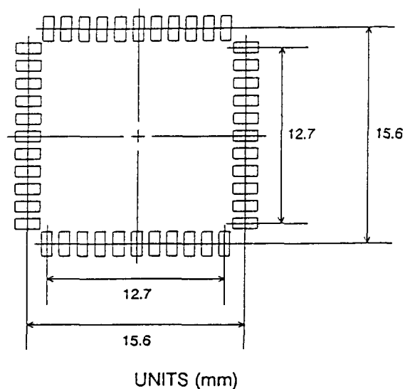
Figure 6. Pad Placement
