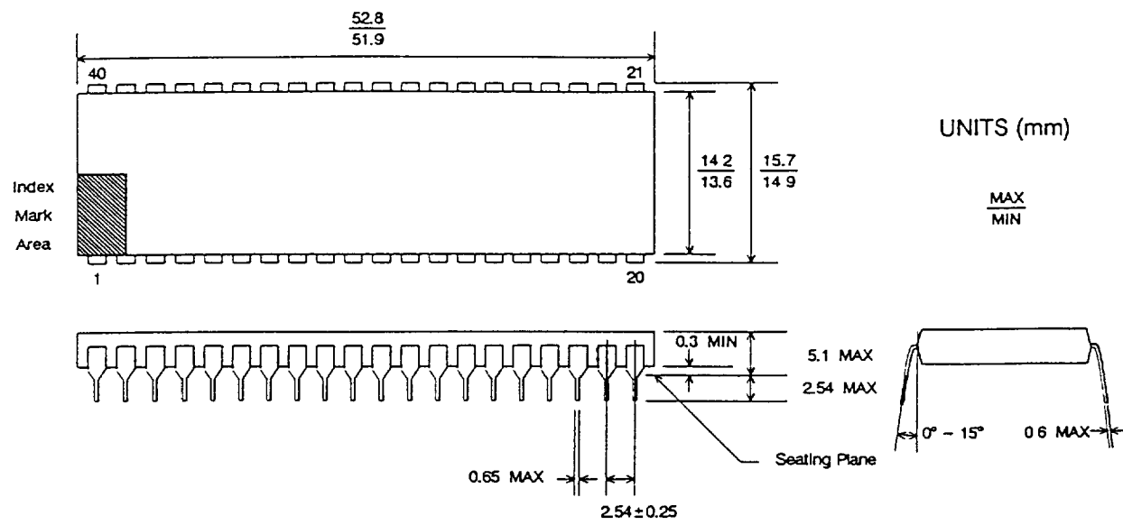
Figure 3. HBCR-1800, -1810, -2000, -2010
