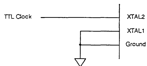
Figure 10. 1800, 1801, 2000, 2001 ICs
