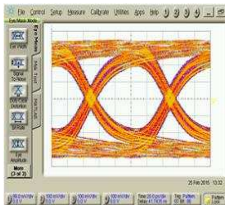
Figure 10. 10 Gbps Output Eye Diagram
