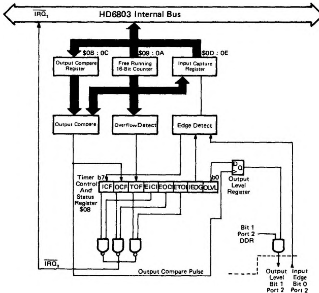
Figure 13 Block Diagram of Programmable Timer
