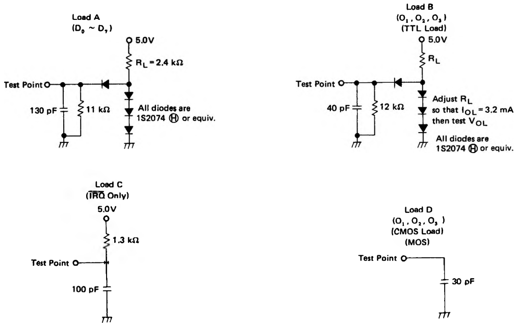
Figure 8 Test Loads
