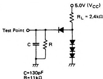
Figure 14 Bus Timing Test Loads
