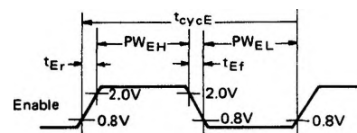
Figure 11 Enable Signal Characteristics
