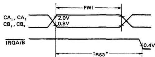
Figure 8 Interrupt Pulse Width and \overline{\text{IRQ}} Response
