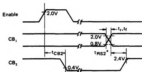
Figure 7 CB 2 Delay Time (Write Mode; CRB5=1, CRB3=CRB4=0)
