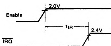
Figure 9 IRQ Release Time
