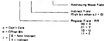
Figure 16 Index Addressing Postbyte Register Bit Assignments
