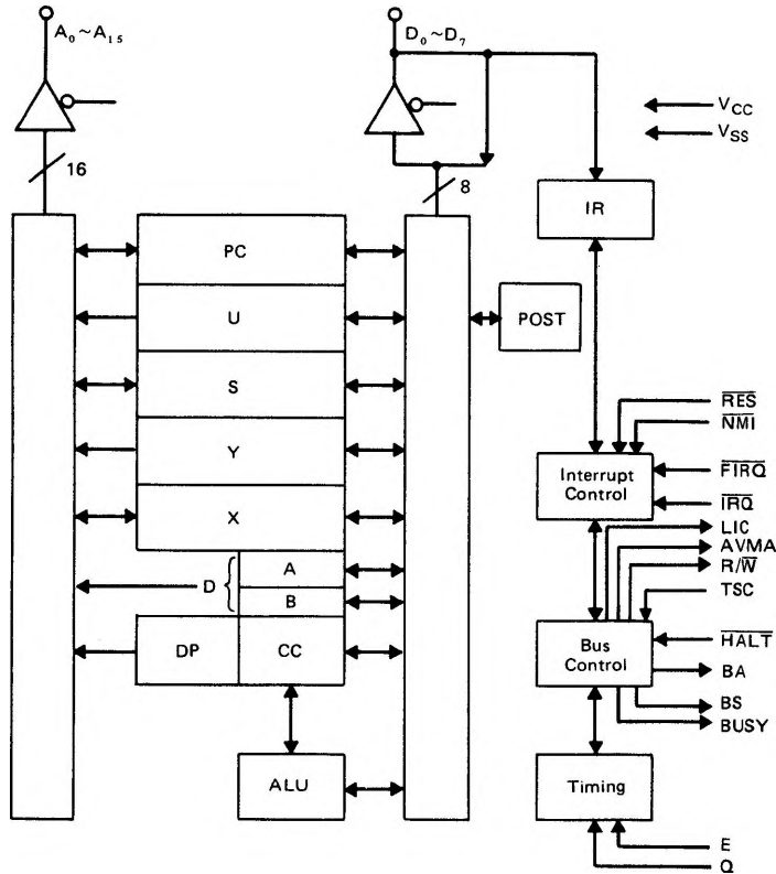
Figure 3 HD6809E Expanded Block Diagram
