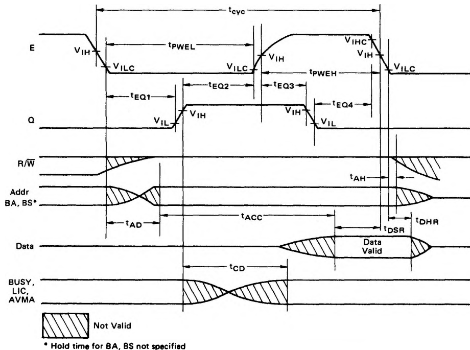
Figure 1 Read Data from Memory or Peripherals
