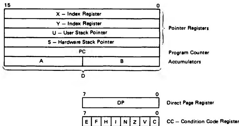
Figure 5 Programming Model of The Microprocessing Unit
