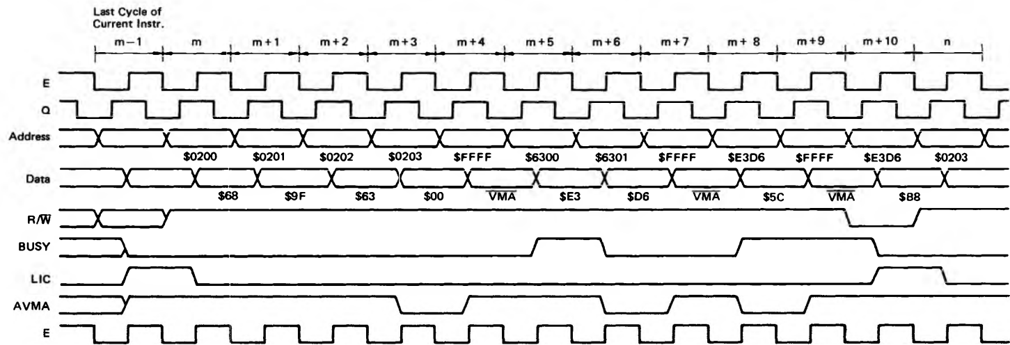
Figure 13 BUSY Timing
