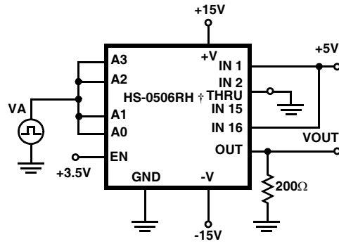
FIGURE 1. BREAK-BEFORE-MAKE DELAY ( t_{OPEN} )
