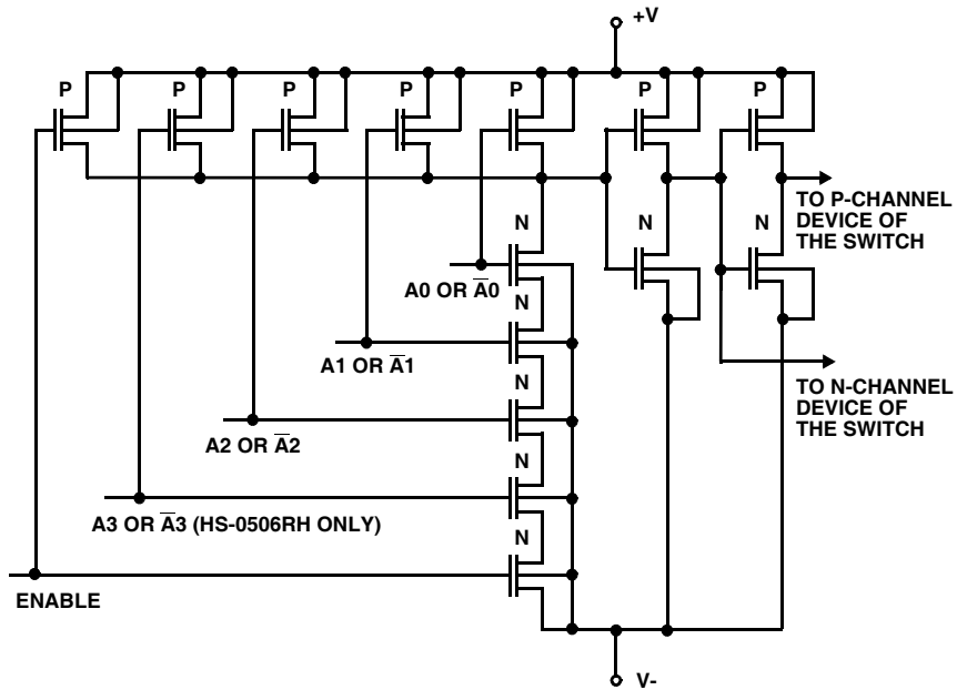
FIGURE 4. ADDRESS DECODER
