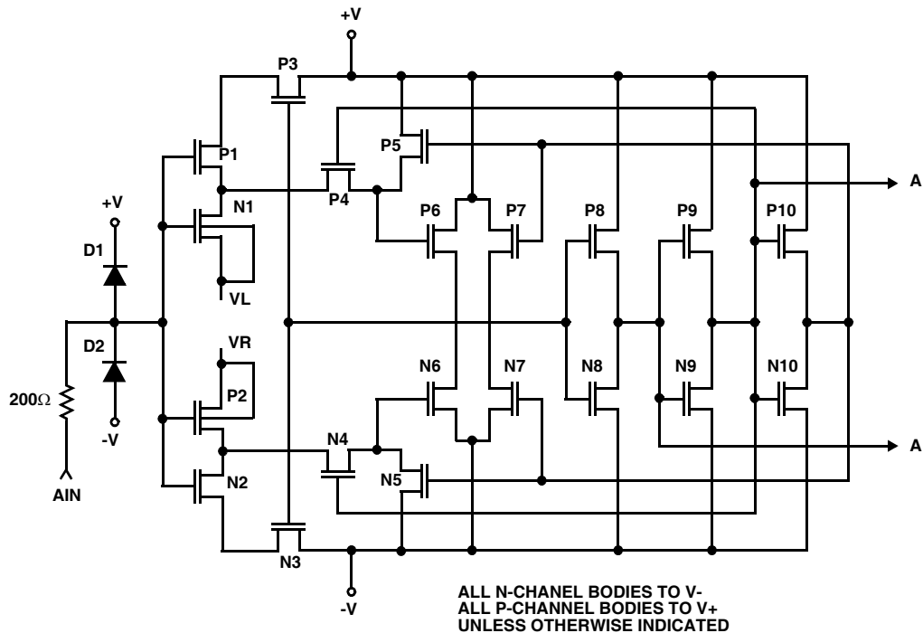
FIGURE 5. ADDRESS INPUT BUFFER LEVER SHIFTER
