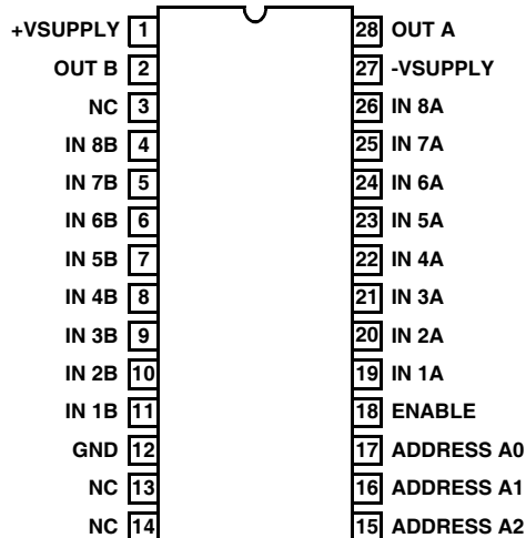
HS-0507RH 28 LEAD CERAMIC DUAL-IN-LINE FRIT SEAL PACKAGE (CerDIP) MIL-STD-1835 GDIP1-T28
