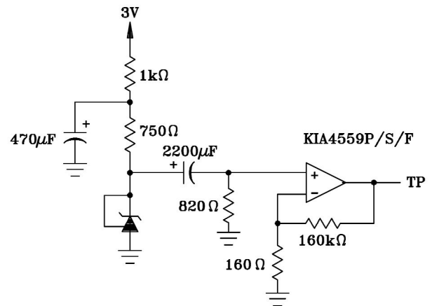
TEST CIRCUIT FOR EQUIVALENT NOISE VOLTAGE
