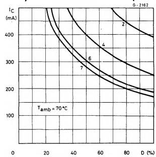
Fig. 11 - Peak collector current as a function fo duty cycle and number of outputs
