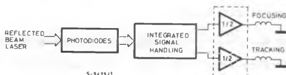
Fig. 9 – Servocontrol for compact-disc
