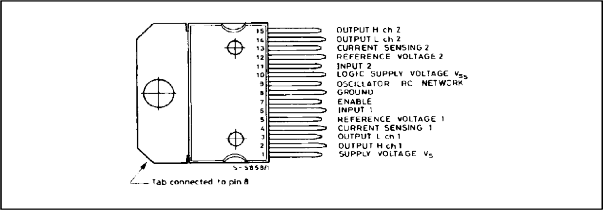
CONNECTION DIAGRAM (top view)
