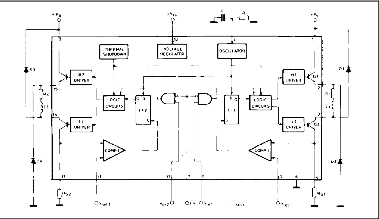
BLOCK DIAGRAM
