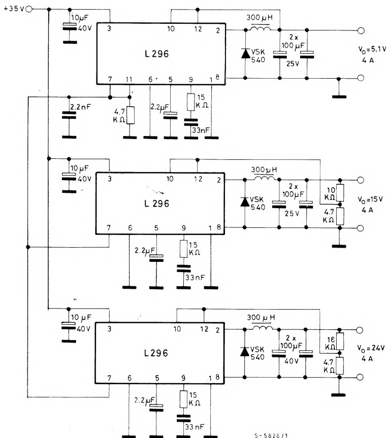
Fig. 15 - Multiple supply
