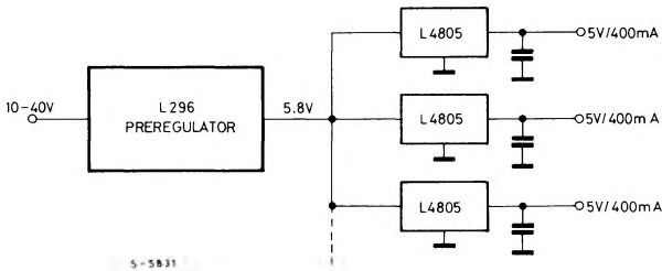
Fig. 14 - Preregulator for distributed supplies
