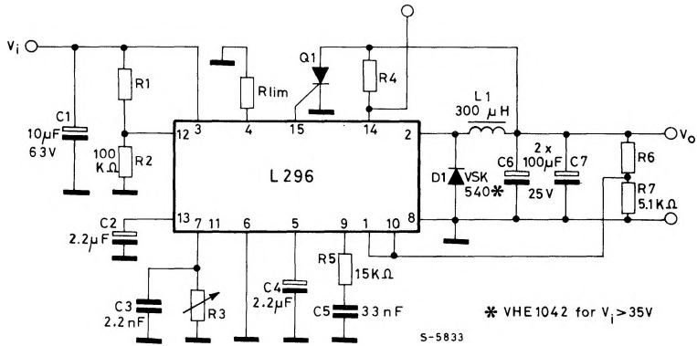
Fig. 4 - Test circuit
