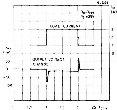
Figure 18 : Load Transient Response (see fig. 4).
